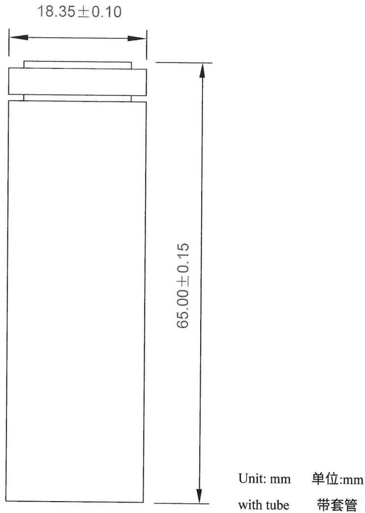
Fig. 1. Outline Dimensions of INR18650/25P
